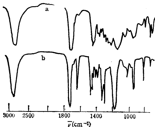
Fig. 1 IR spectrum of monomer and polymer a. Monomer; b. Polymer
