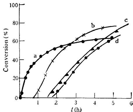
Fig. 4 Time-conversion curve for different [cat]/[I]
