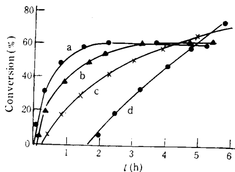
Fig. 5 Time-conversion curves for different temperature
