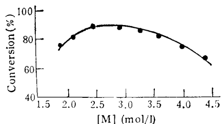
Fig. 8 The effect of monomer concentration on conversion [\text{M}]/[\text{I}] = 56.9 , [\text{cat}]/[\text{I}] = 0.026 , T = 80^\circ\text{C} Solvent: Ligarine
