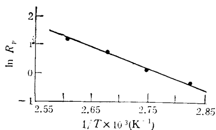
Fig. 7 \ln R_p versus 1/T polymerization conditions are the same as Fig. 5
