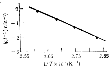
Fig. 6 \lg t^{-1} versus 1/T polymerization conditions are the same as Fig. 5
