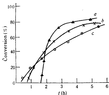
Fig. 2 Time-conversion curves for different initiator concentration
